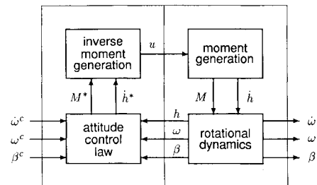
Fig. 1 Simplified attitude controller (left half) and vehicle (right half).
