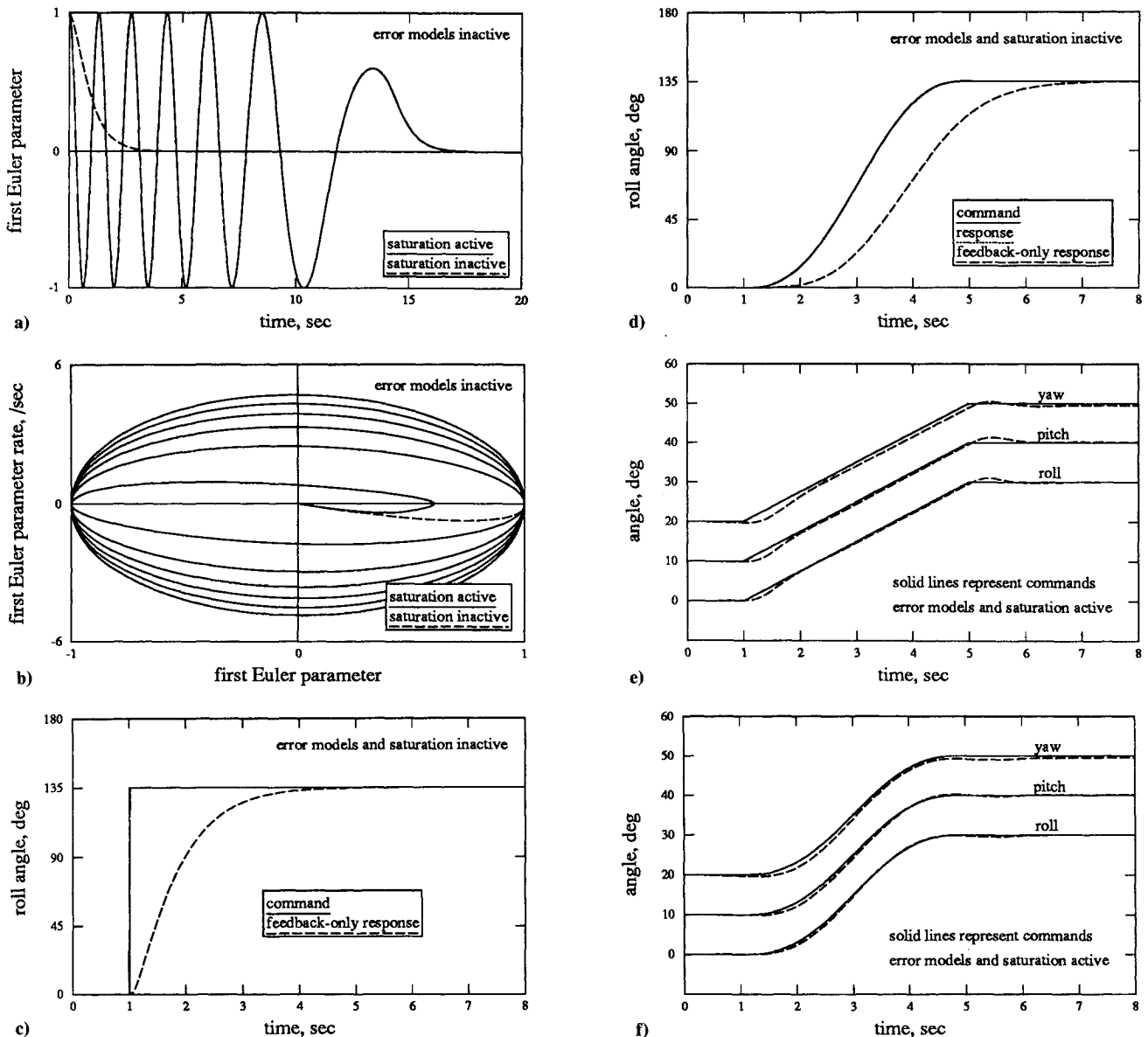
Fig. 3 Simulation results: a) time response for attitude acquisition; b) phase-plane diagram for attitude acquisition; c) time response for step command; d) time response for continuous command; e) time response for continuous multi-axis commands; and f) time response for continuous multi-axis commands.
