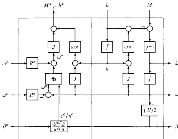
Fig. 2 Attitude control law (left half) and vehicle rotational dynamics (right half).
